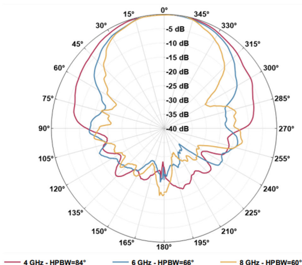
Typical Frequency Point Radiation Patterns
