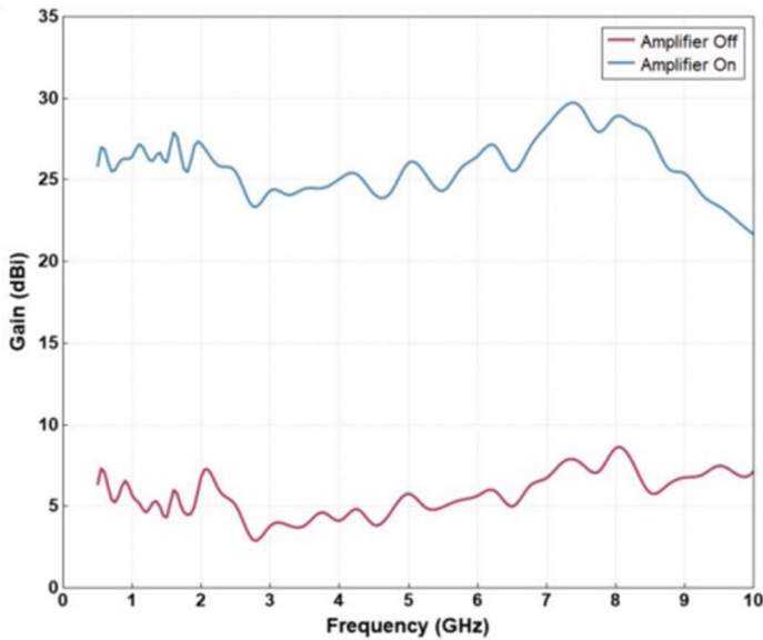
Gain
