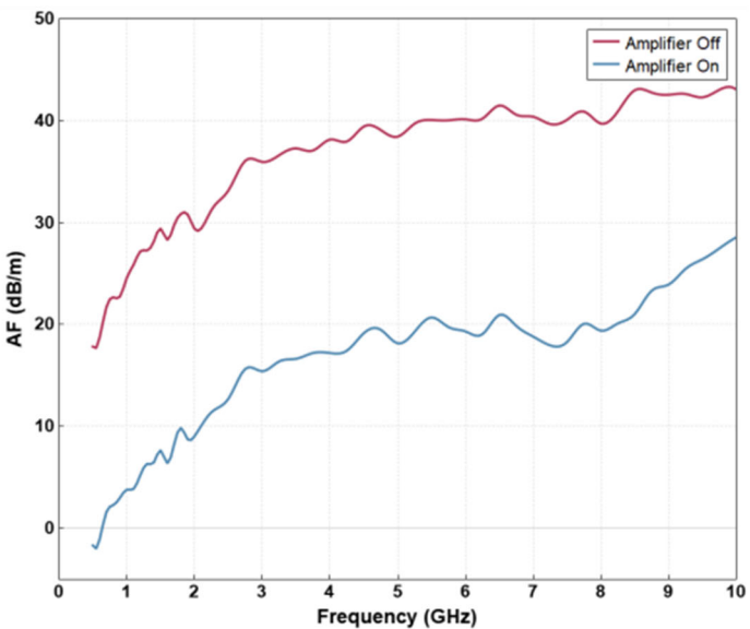
Antenna Factor
